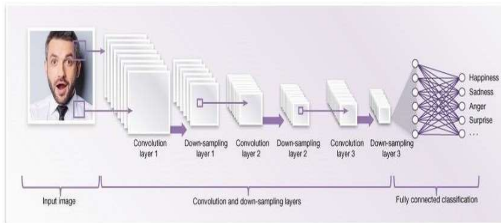
Figure 3 CNN architecture
